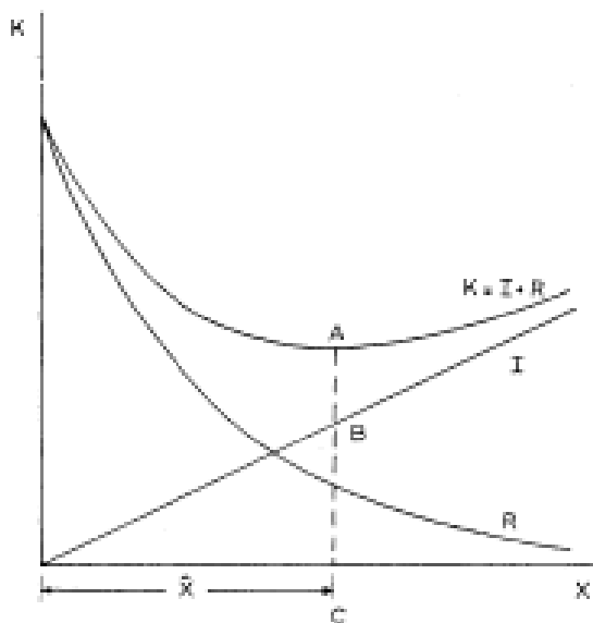
Figure 3.2 Minimizing total costs (K) from raising a dike (I) and expected economic damage (R) (figure 3.1.3 in Dantzig and Kriens, 1961).
