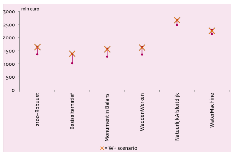
Figure 5.1 Sensitivity of the costs of six basic alternatives for renovating the Afsluitdijk (Zuiderzee-enclosure dam) for different assumption about the rise in the sea level.
